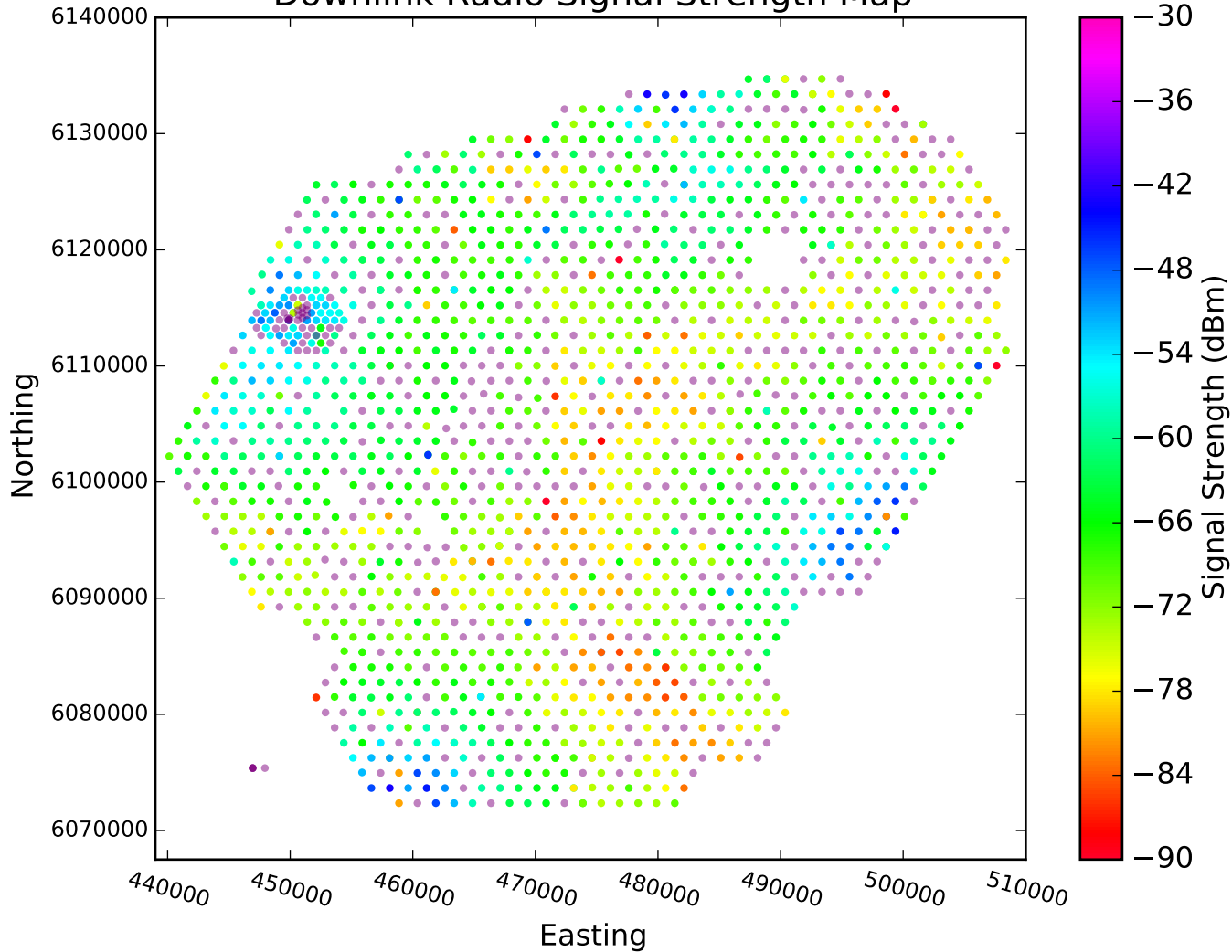
Downlink Radio Signal Strength Map
