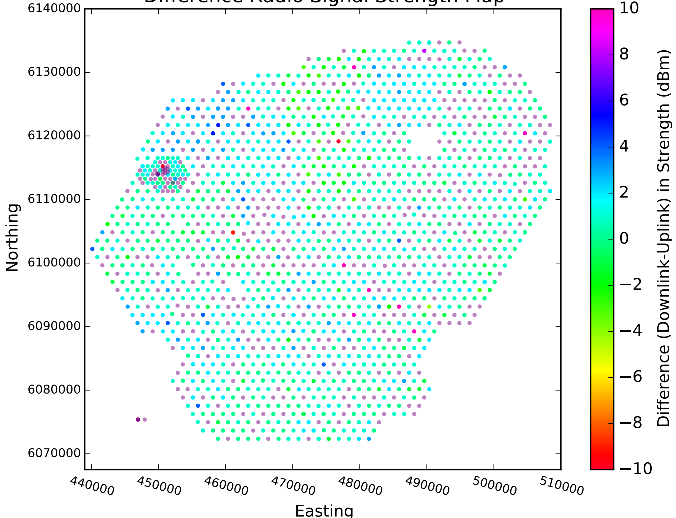
Difference Radio Signal Strength Map
