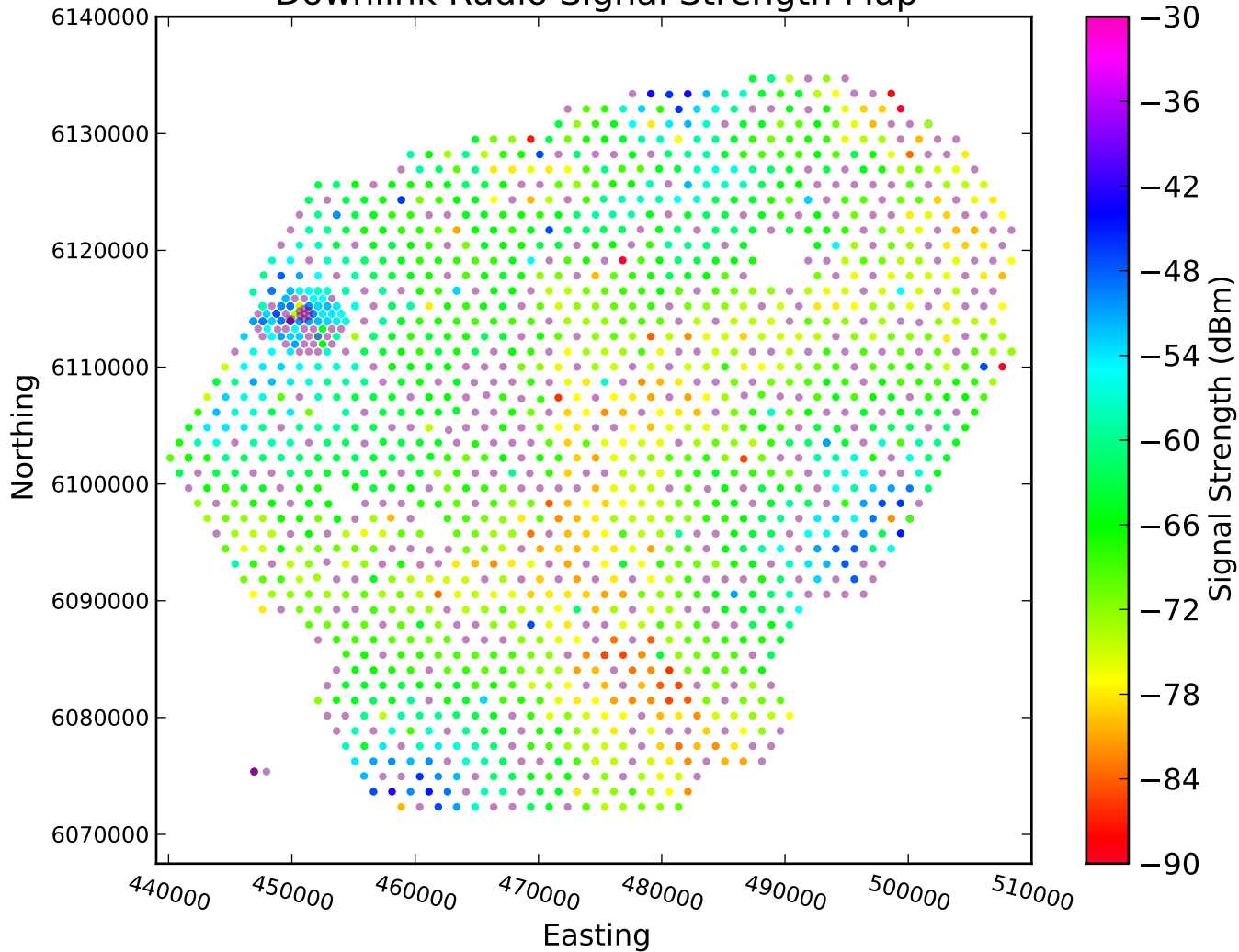
Downlink Radio Signal Strength Map
