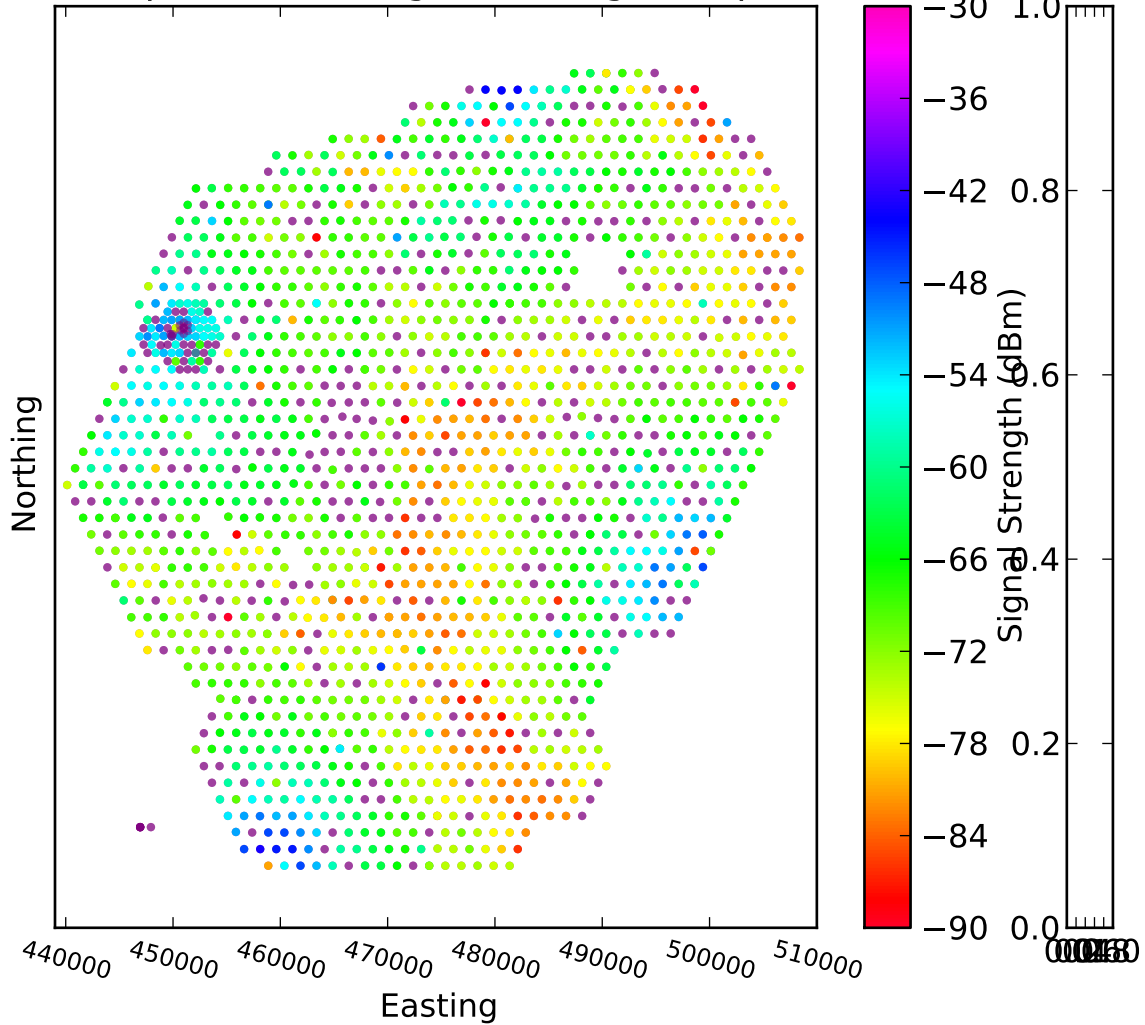
Uplink Radio Signal Strength Map
