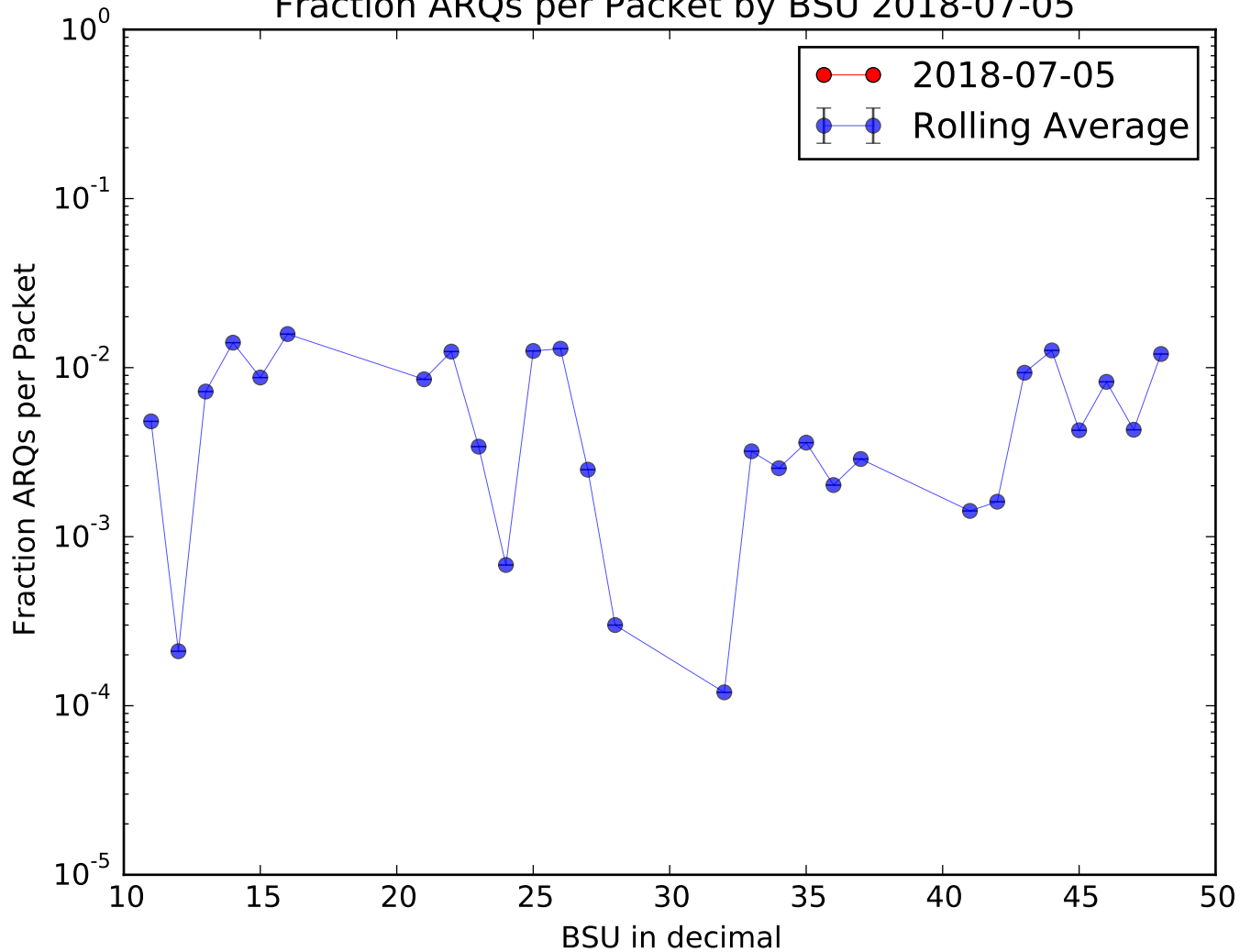
Fraction ARQs per Packet by BSU 2018-07-05
