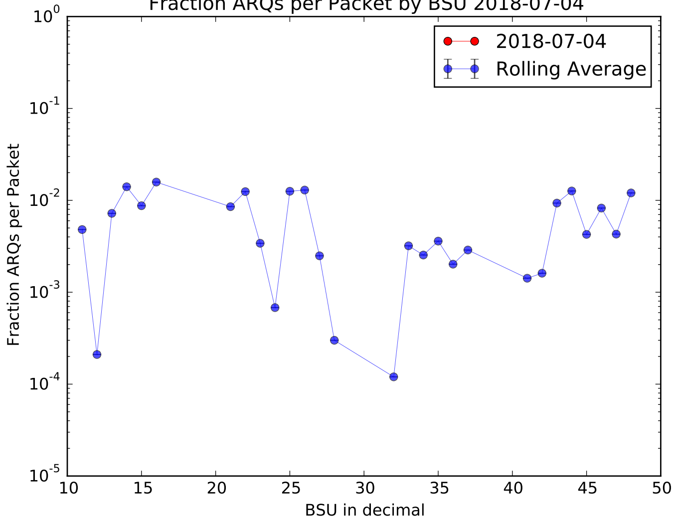
Fraction ARQs per Packet by BSU 2018-07-04
