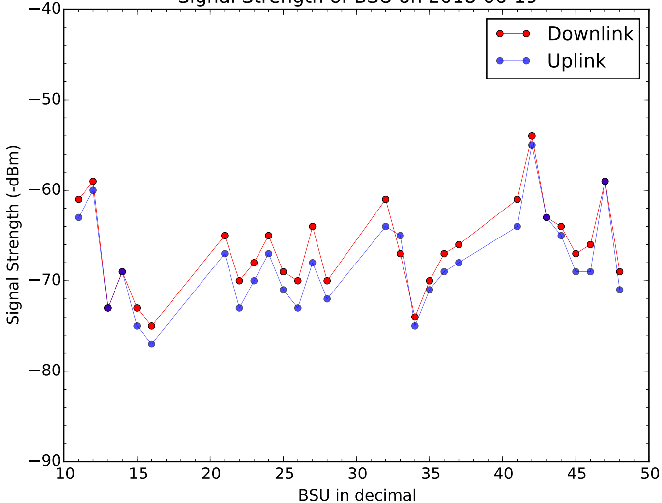
Signal Strength of BSU on 2018-06-19
