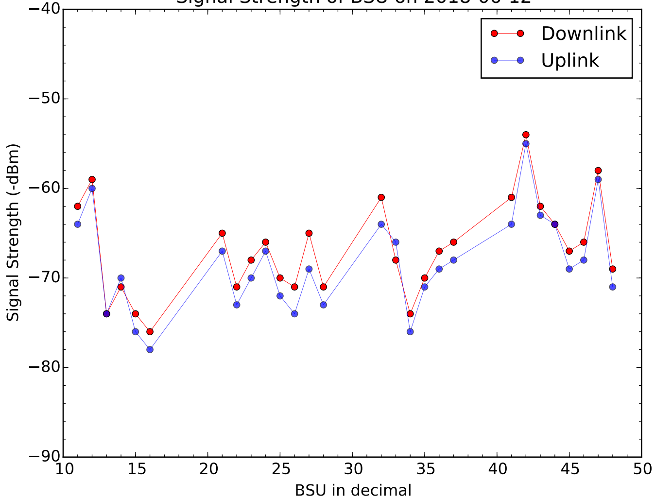
Signal Strength of BSU on 2018-06-12
