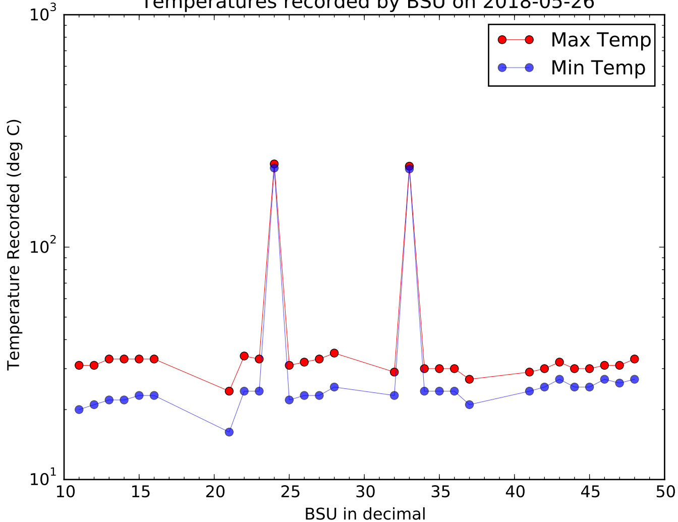
Temperatures recorded by BSU on 2018-05-26
