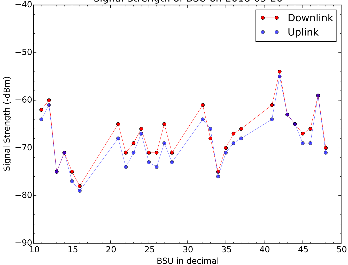
Signal Strength of BSU on 2018-05-20
