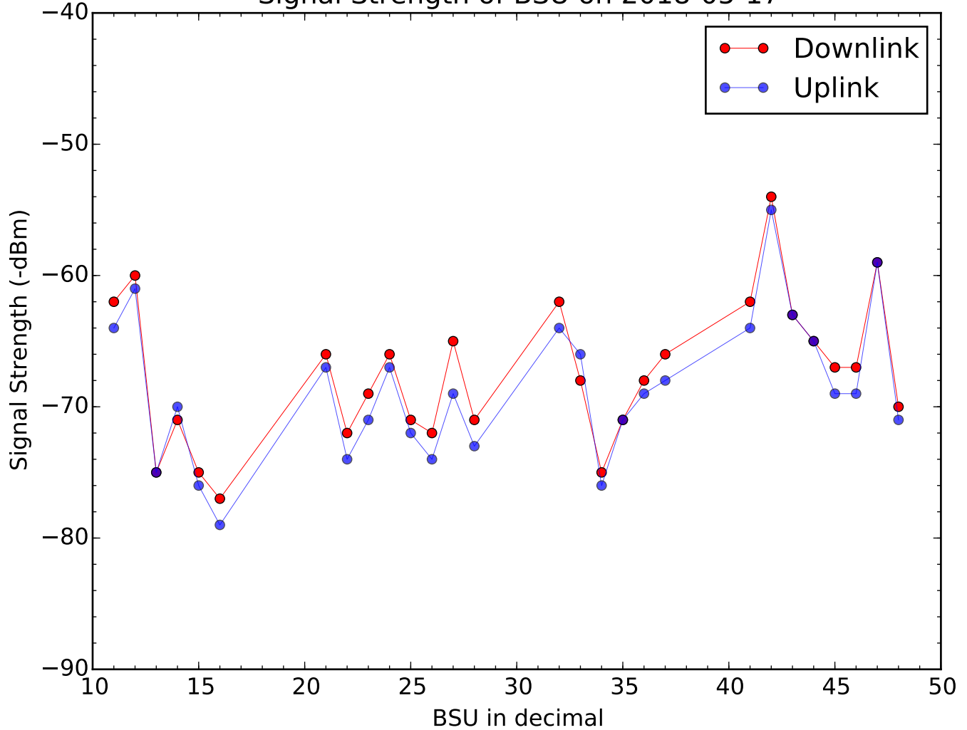
Signal Strength of BSU on 2018-05-17
