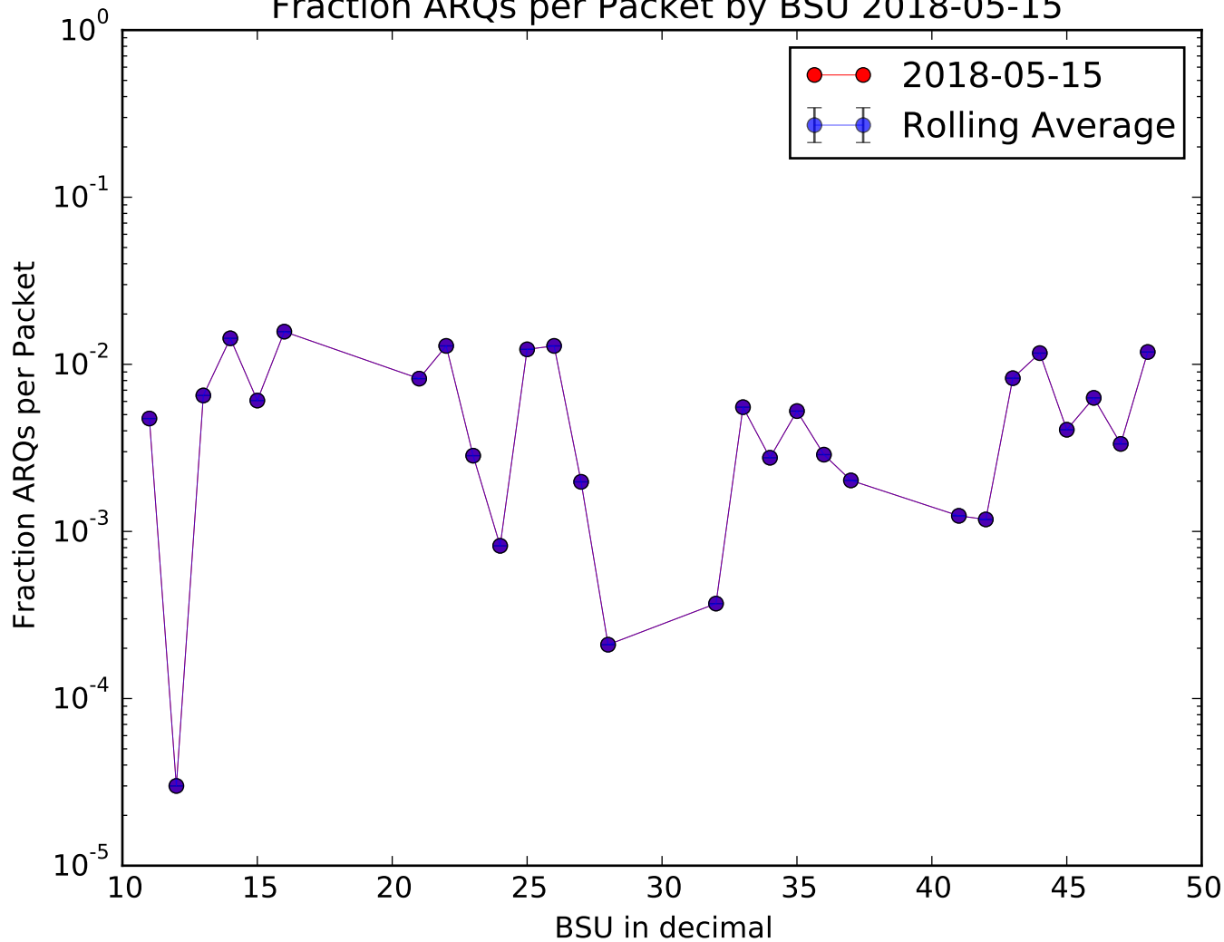
Fraction ARQs per Packet by BSU 2018-05-15
