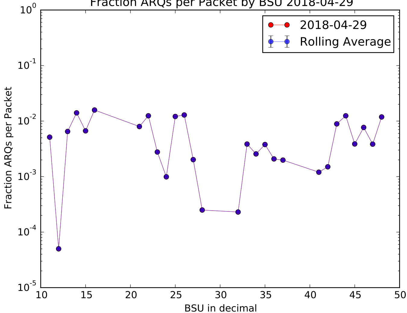
Fraction ARQs per Packet by BSU 2018-04-29
