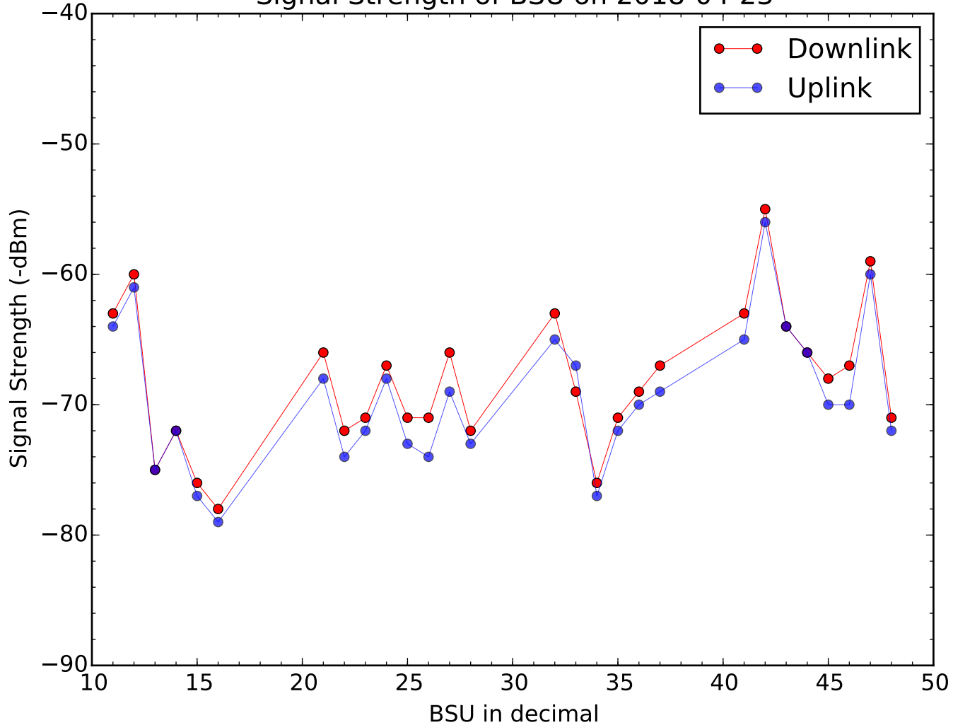
Signal Strength of BSU on 2018-04-23
