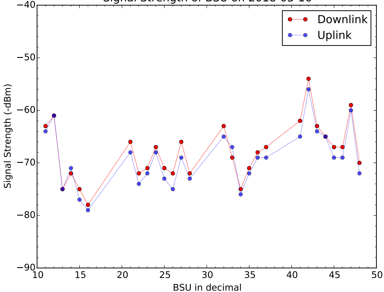
Signal Strength of BSU on 2018-03-16
