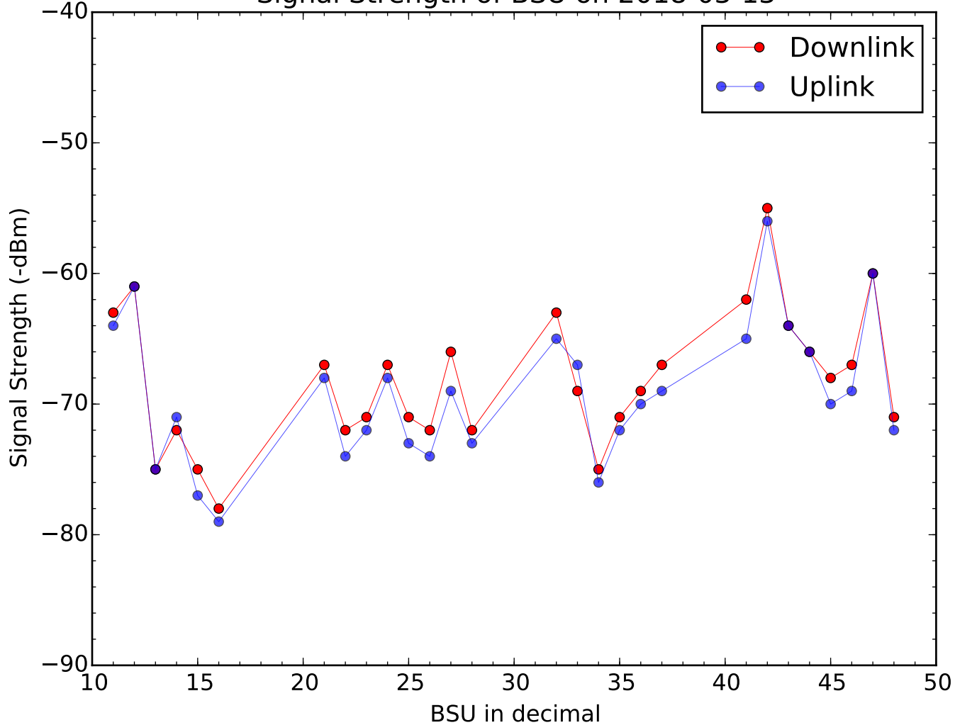
Signal Strength of BSU on 2018-03-13
