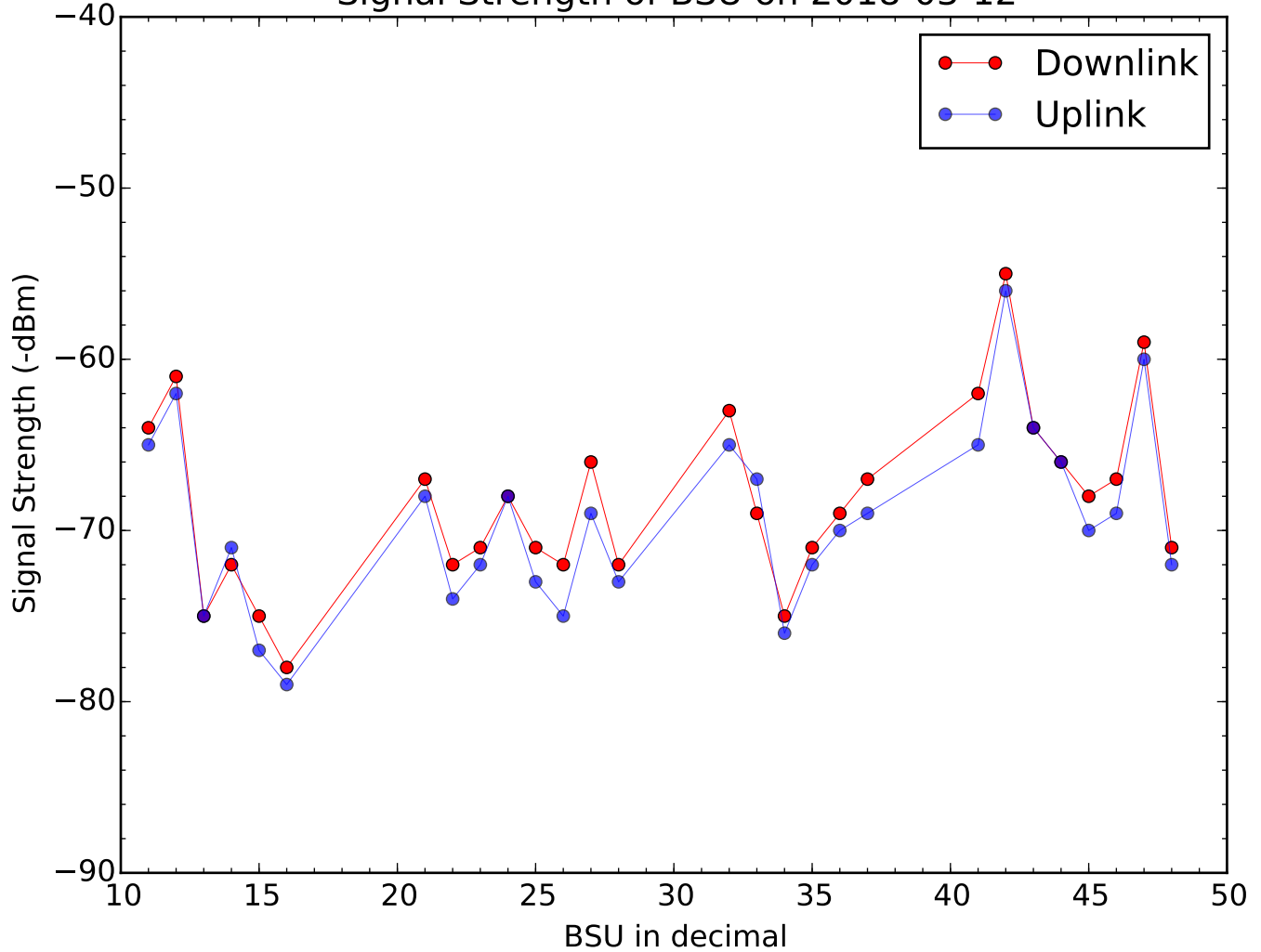
Signal Strength of BSU on 2018-03-12
