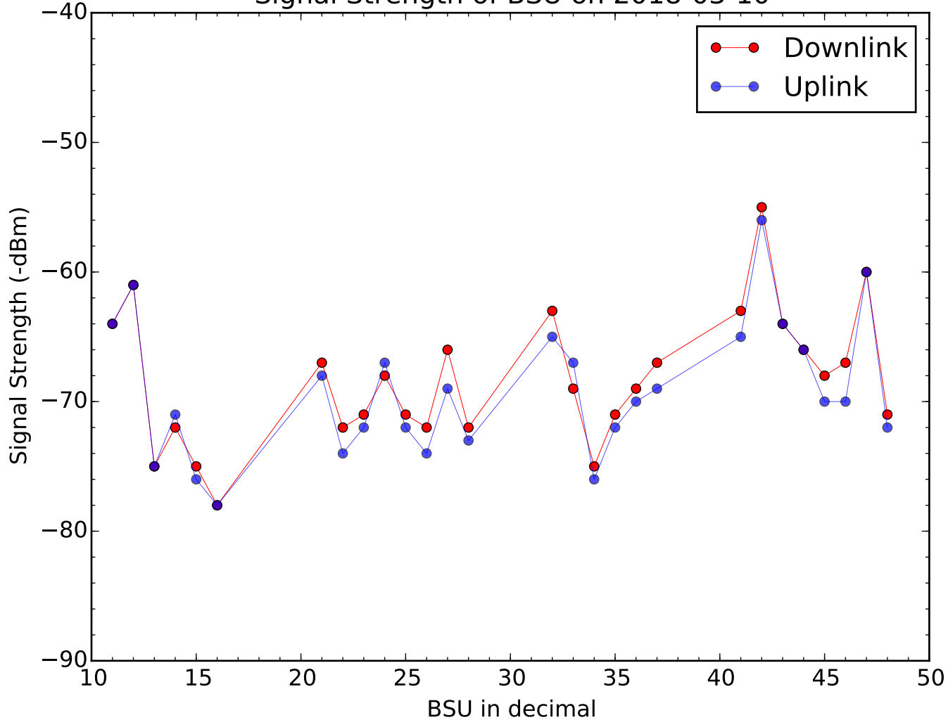
Signal Strength of BSU on 2018-03-10
