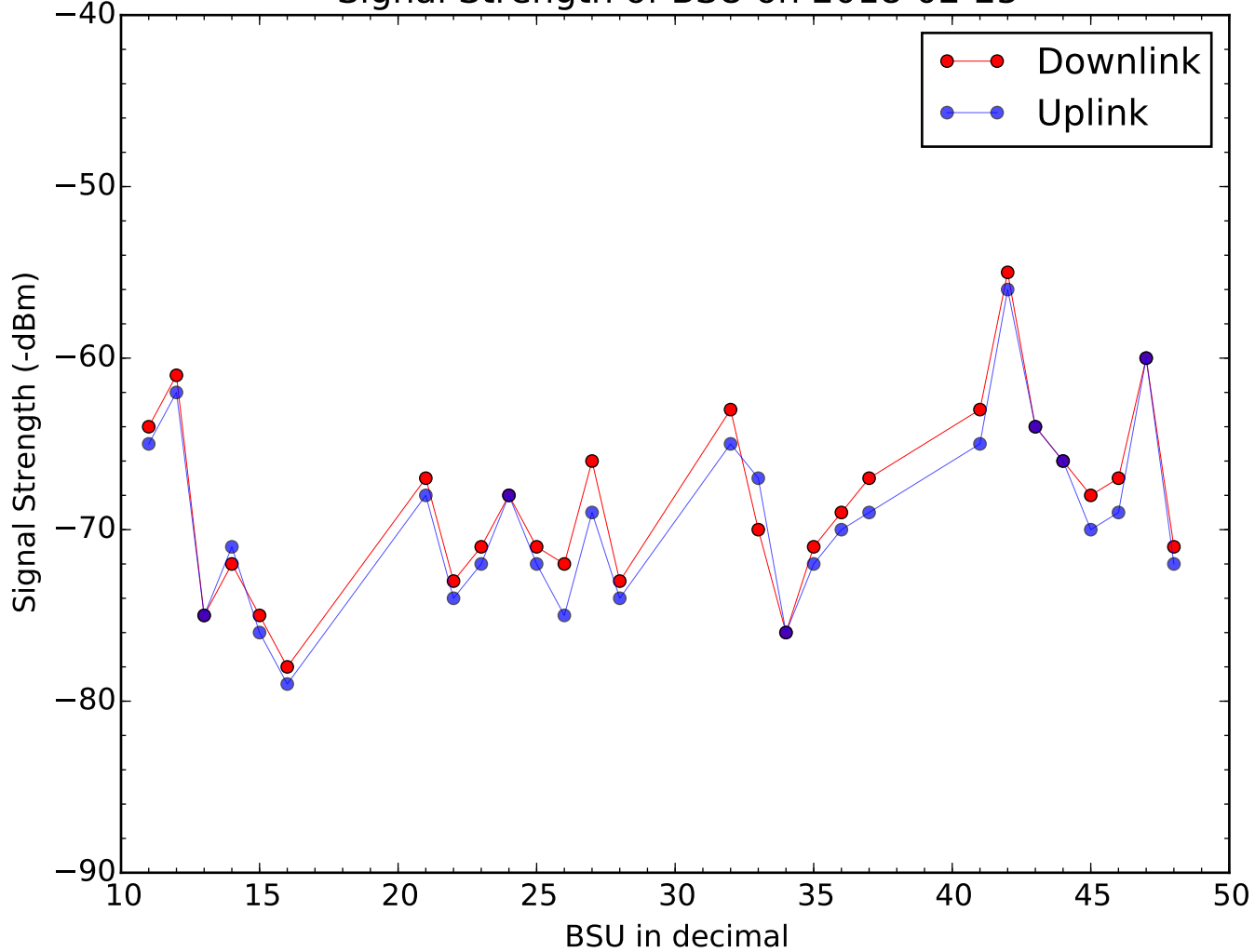
Signal Strength of BSU on 2018-02-25
