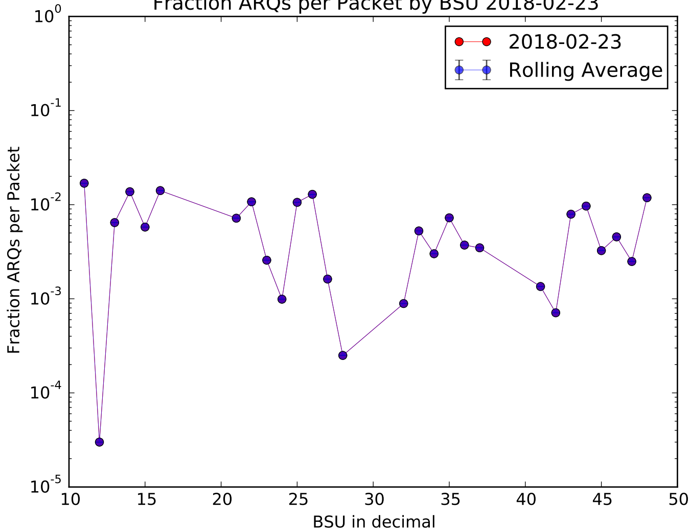
Fraction ARQs per Packet by BSU 2018-02-23
