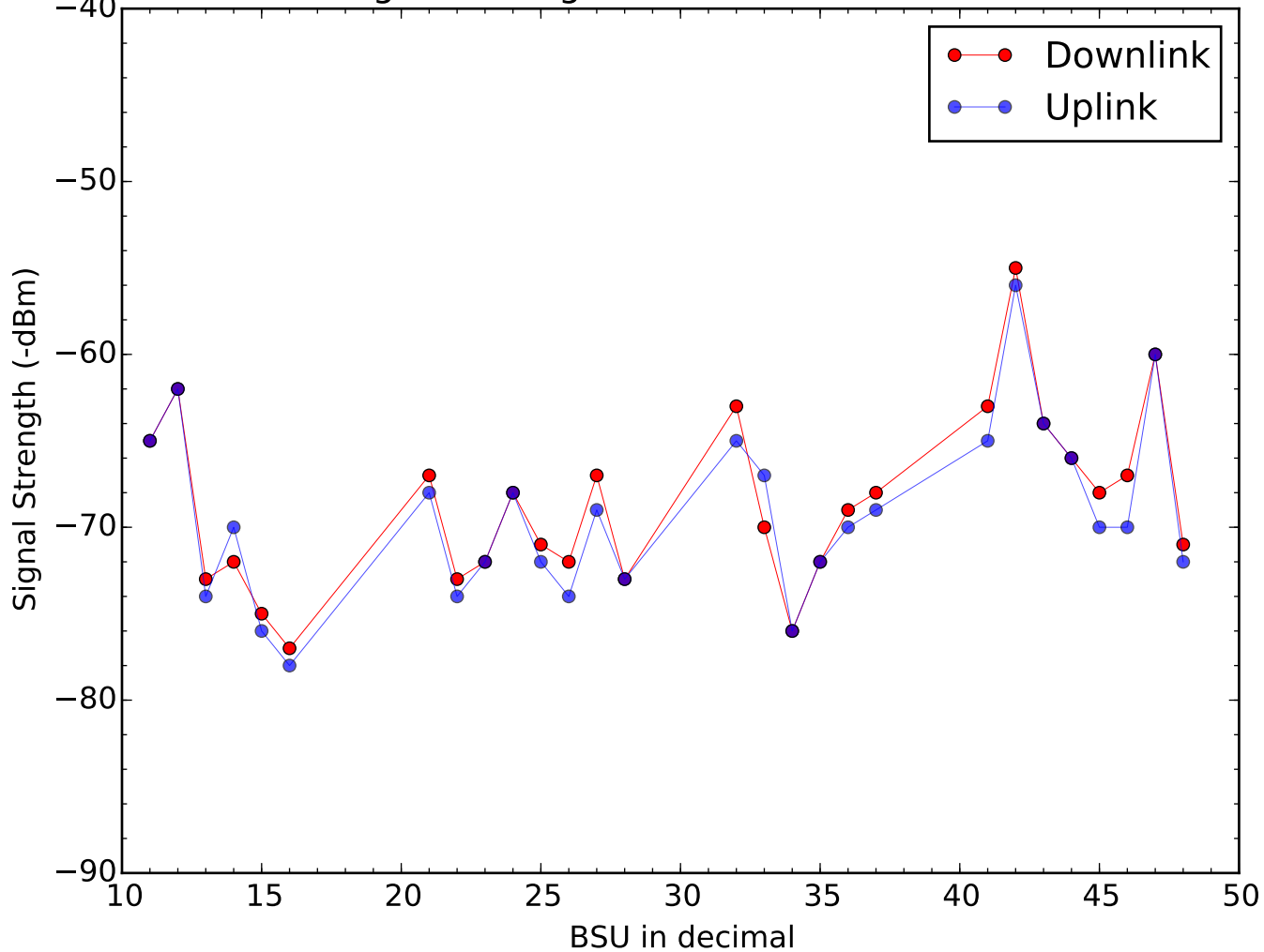
Signal Strength of BSU on 2018-02-19
