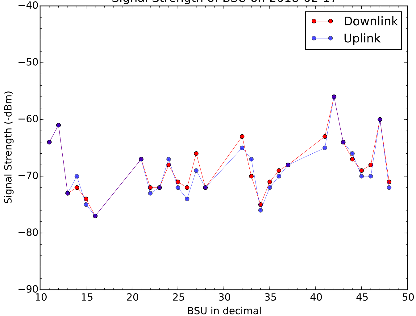
Signal Strength of BSU on 2018-02-17
