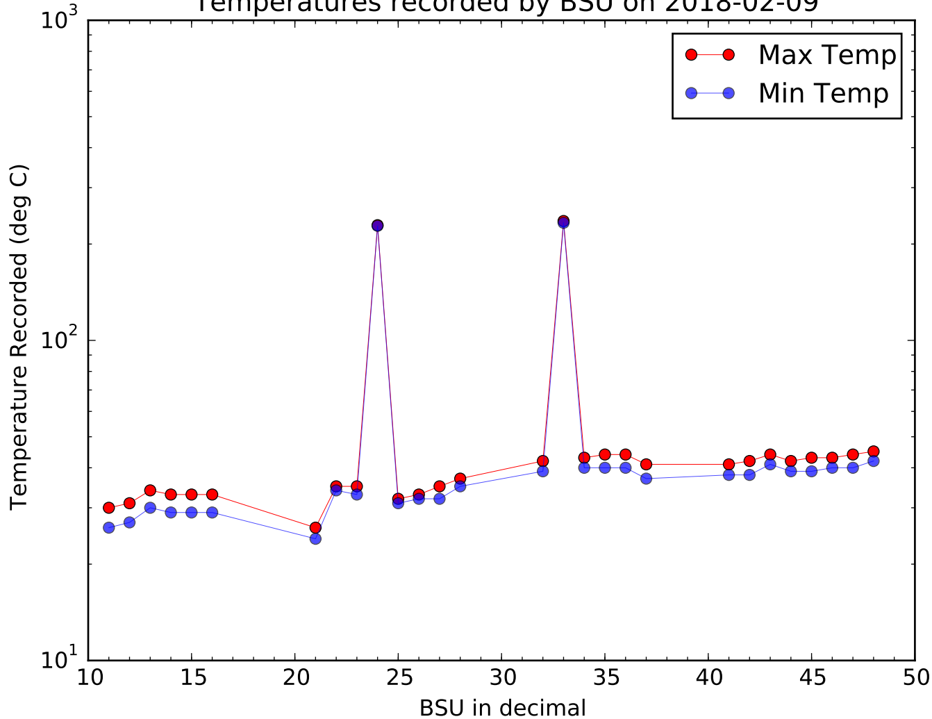
Temperatures recorded by BSU on 2018-02-09
