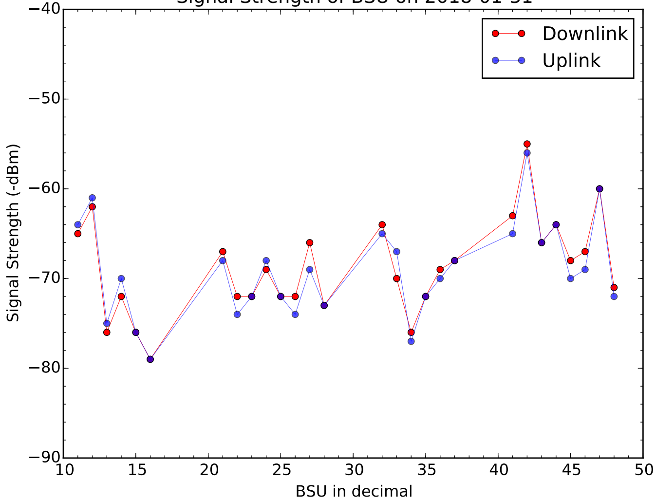
Signal Strength of BSU on 2018-01-31
