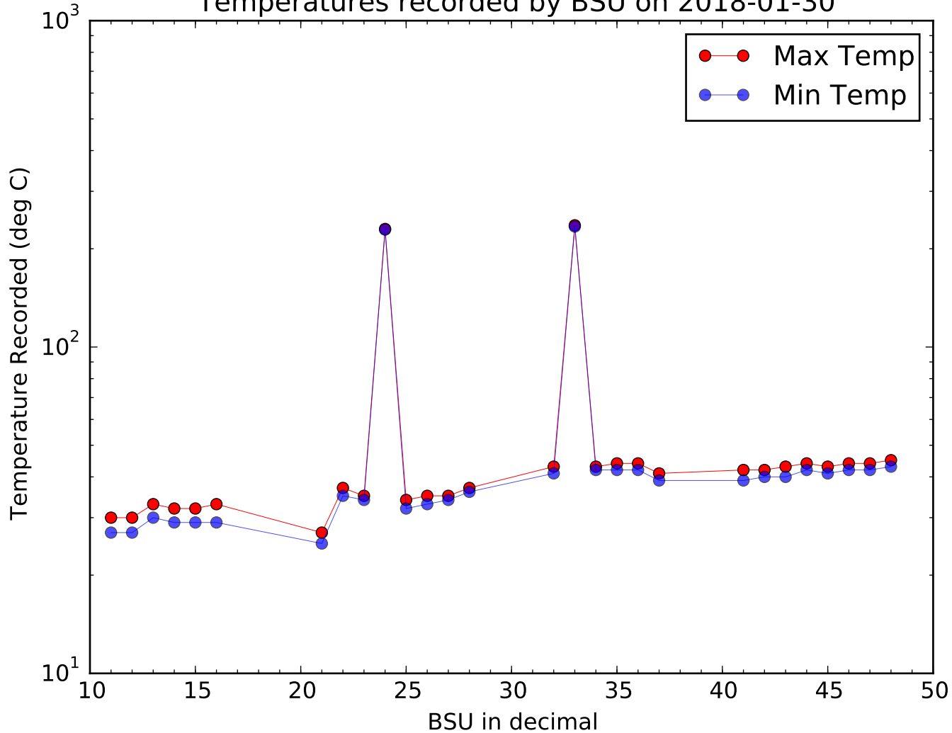
Temperatures recorded by BSU on 2018-01-30
