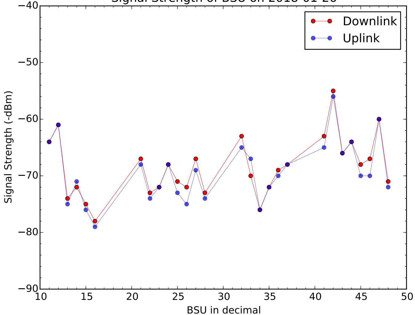
Signal Strength of BSU on 2018-01-26
