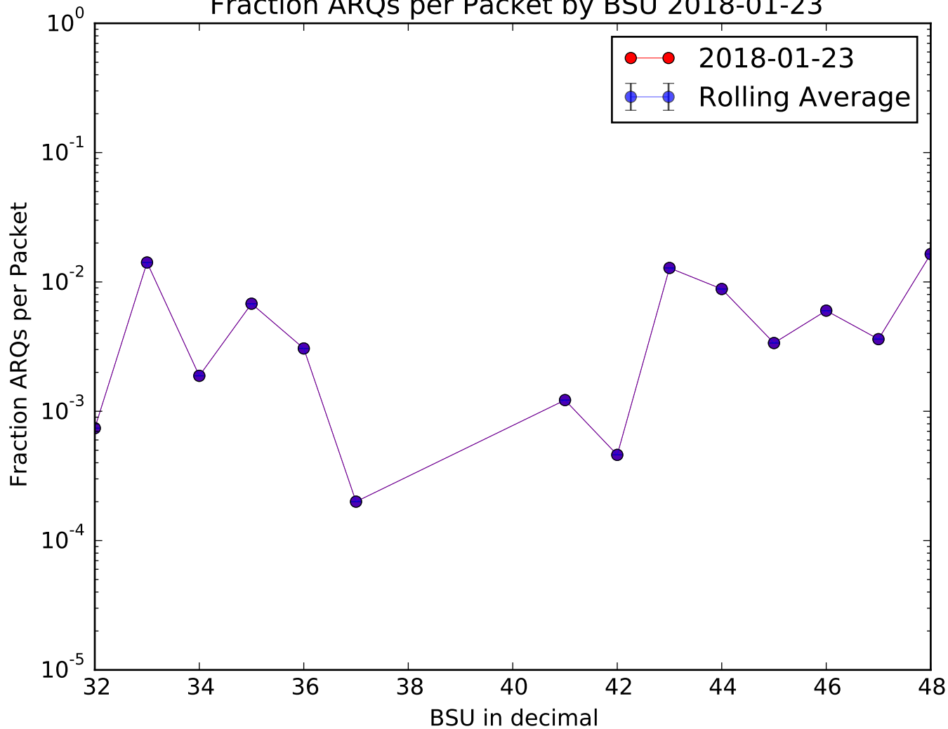
Fraction ARQs per Packet by BSU 2018-01-23
