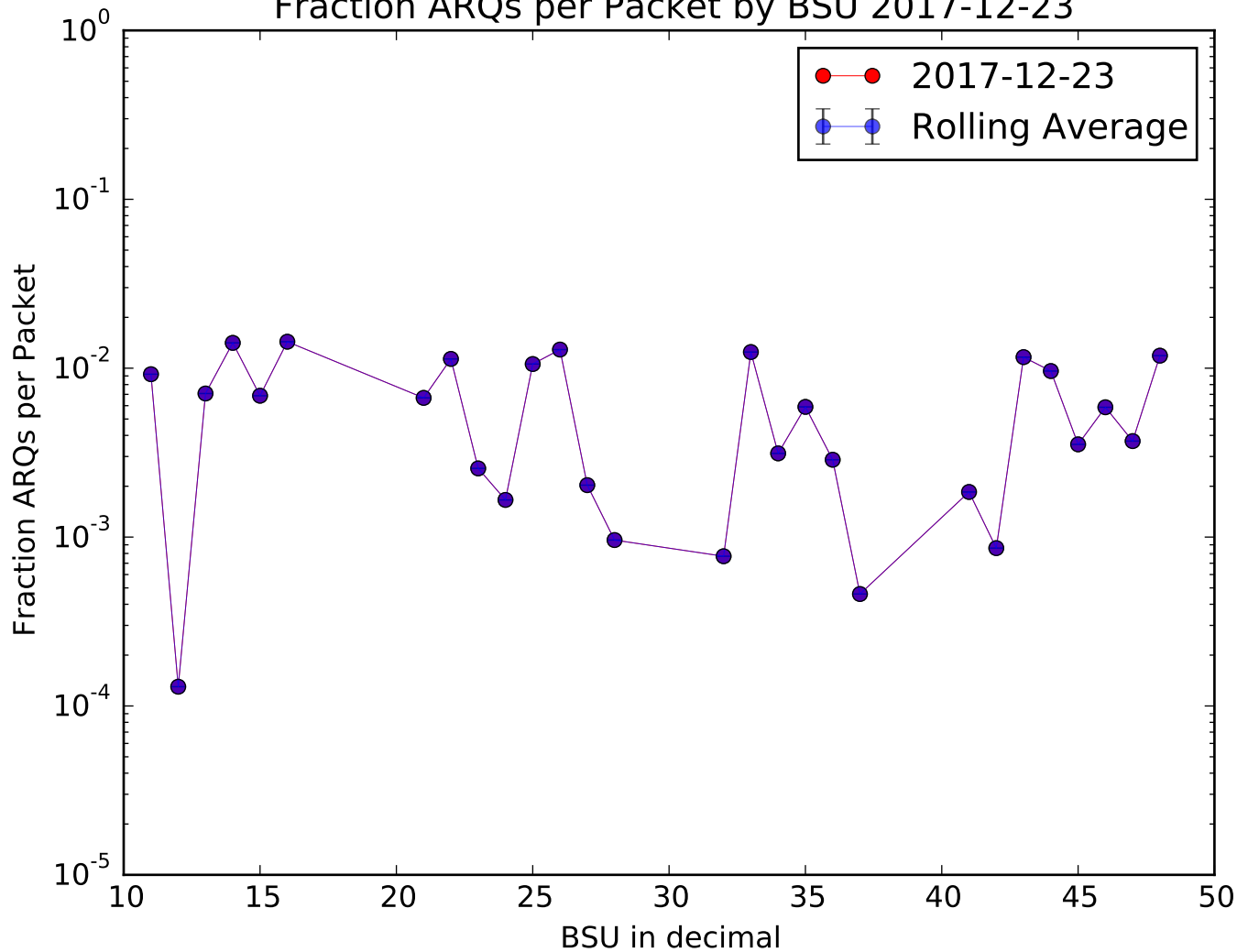
Fraction ARQs per Packet by BSU 2017-12-23
