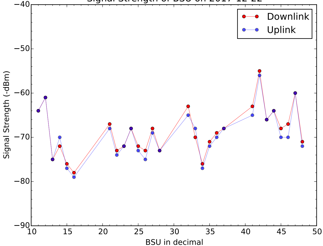
Signal Strength of BSU on 2017-12-22
