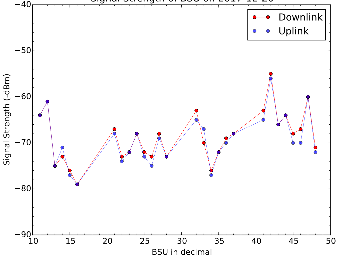
Signal Strength of BSU on 2017-12-20
