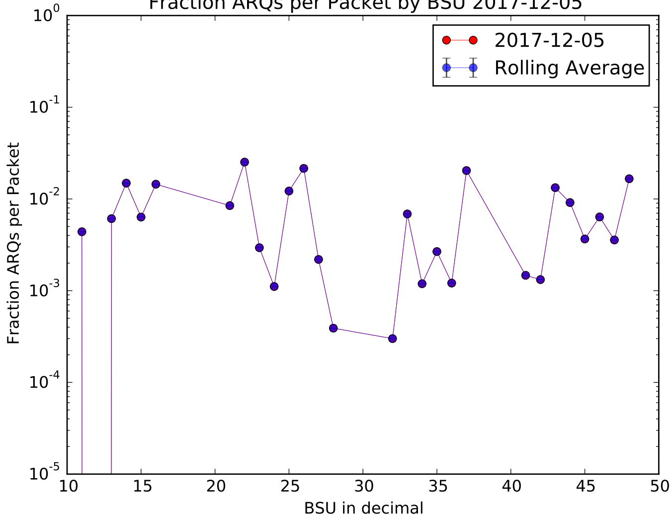
Fraction ARQs per Packet by BSU 2017-12-05
