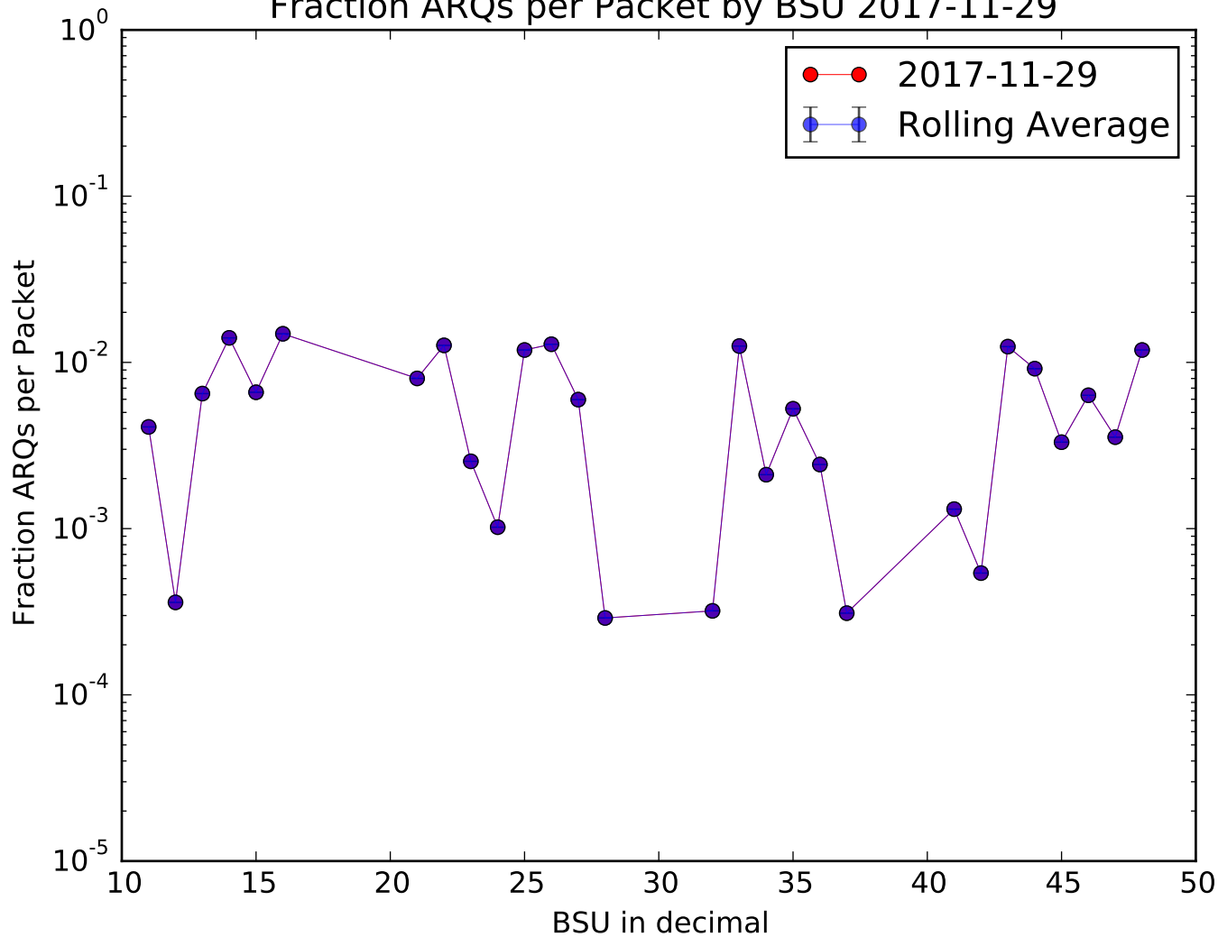
Fraction ARQs per Packet by BSU 2017-11-29
