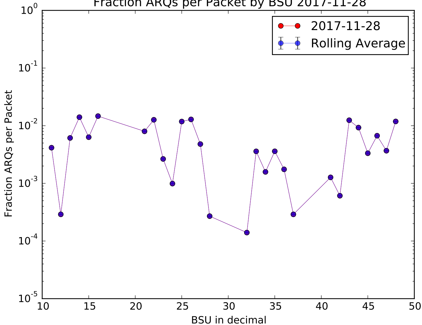
Fraction ARQs per Packet by BSU 2017-11-28
