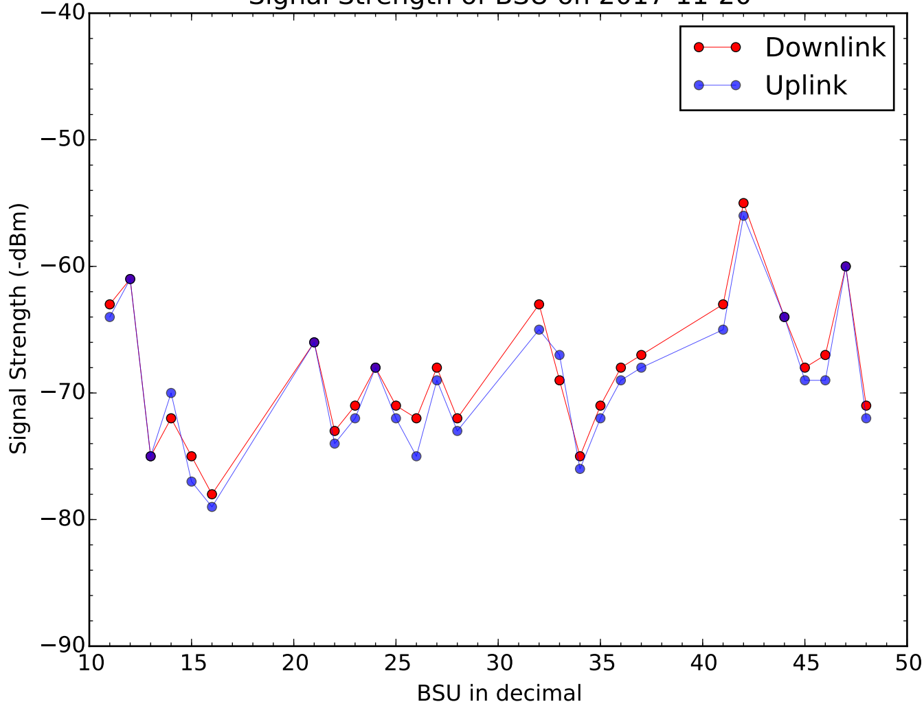
Signal Strength of BSU on 2017-11-20
