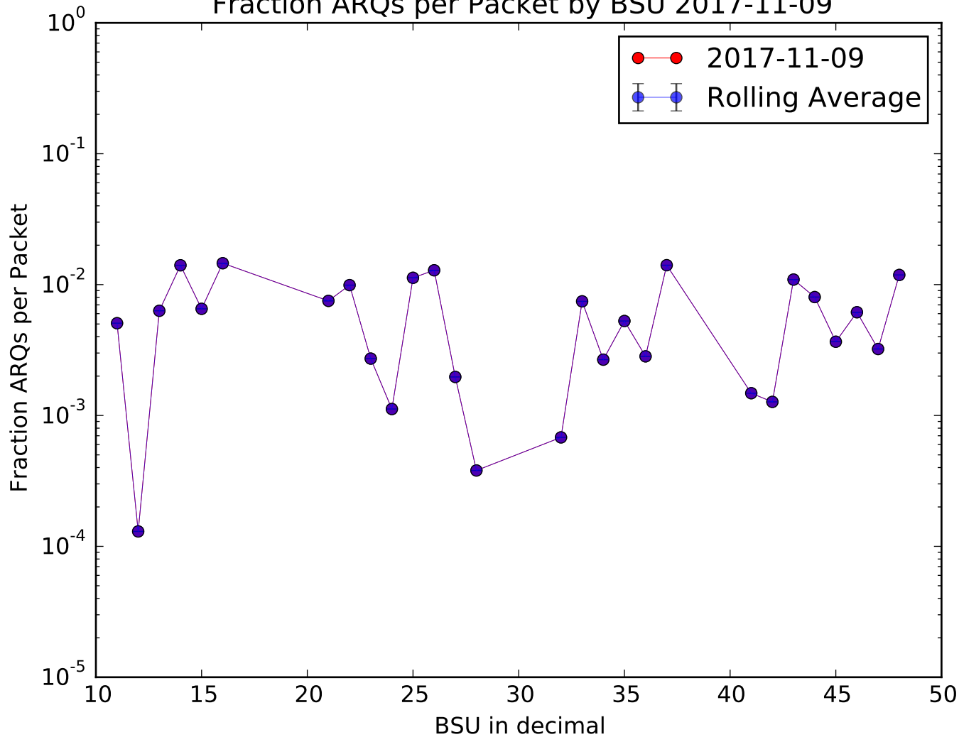
Fraction ARQs per Packet by BSU 2017-11-09
