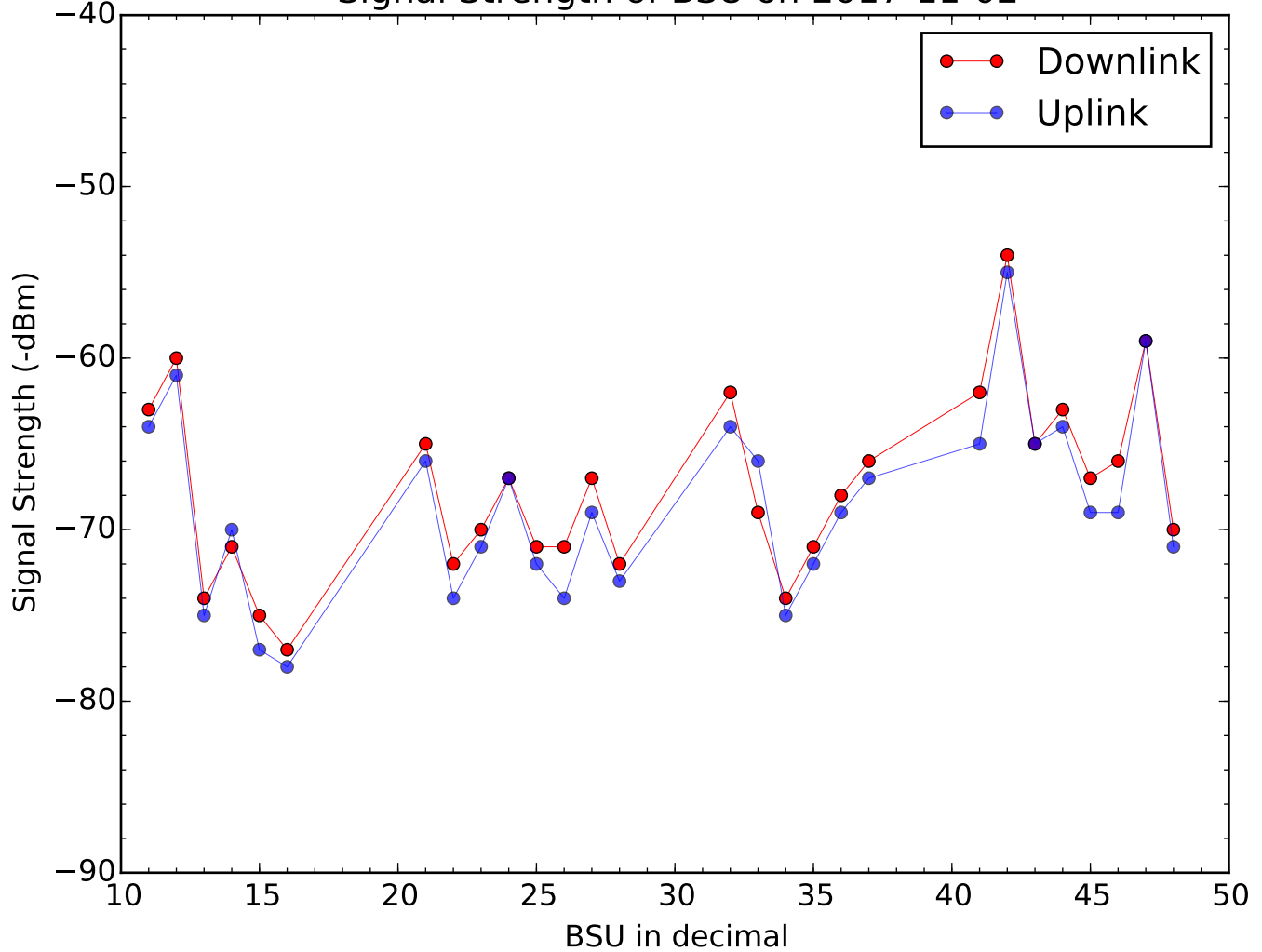
Signal Strength of BSU on 2017-11-02
