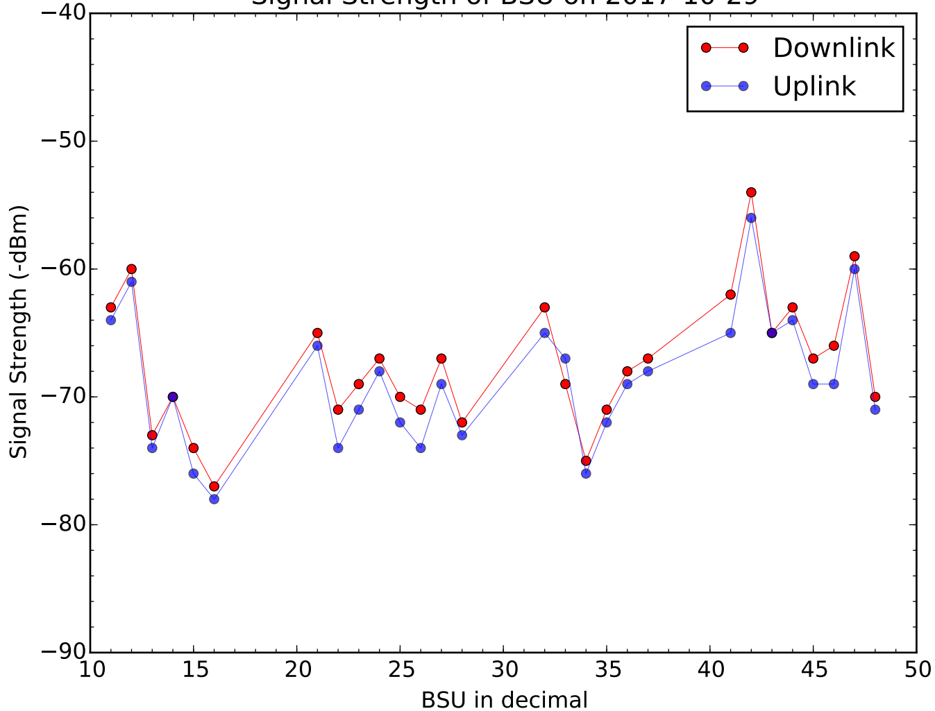
Signal Strength of BSU on 2017-10-29
