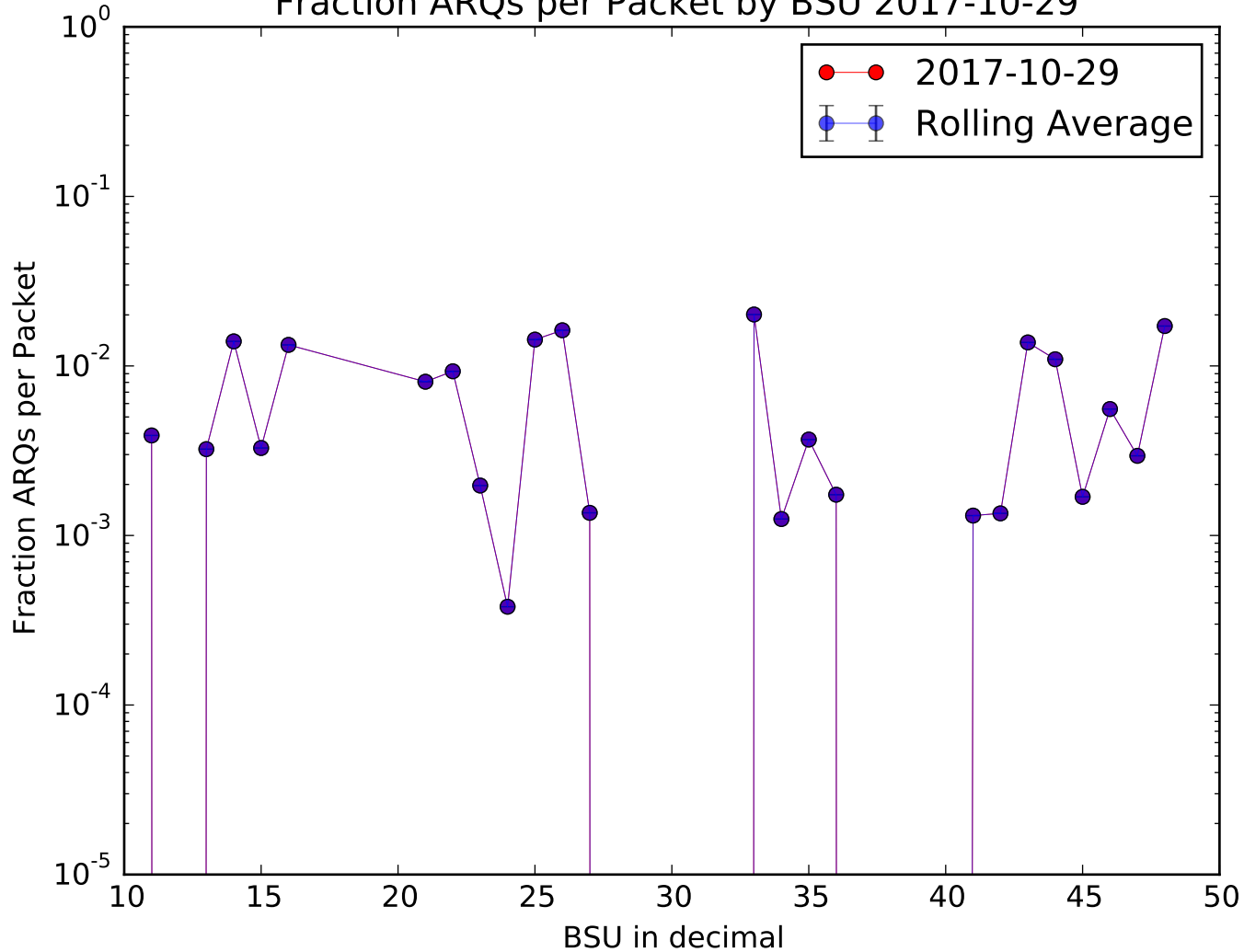
Fraction ARQs per Packet by BSU 2017-10-29
