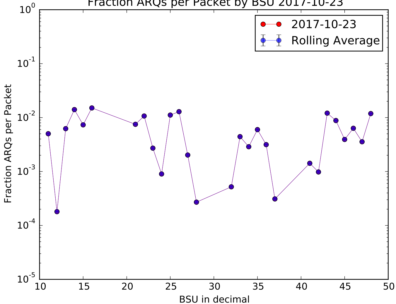
Fraction ARQs per Packet by BSU 2017-10-23
