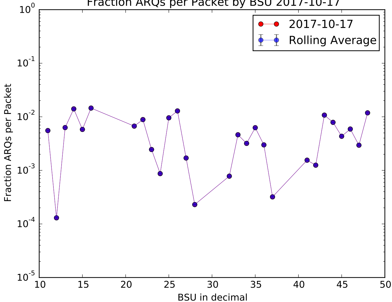
Fraction ARQs per Packet by BSU 2017-10-17
