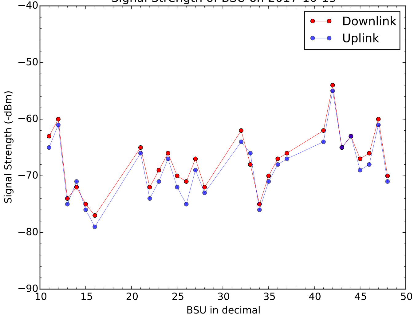
Signal Strength of BSU on 2017-10-13
