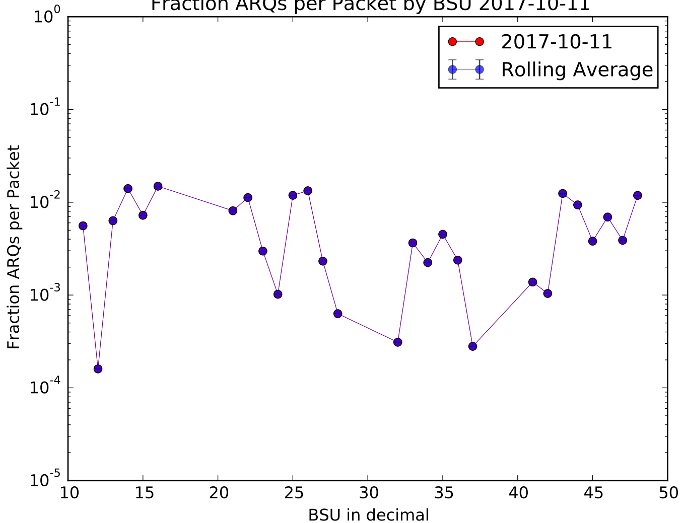
Fraction ARQs per Packet by BSU 2017-10-11
