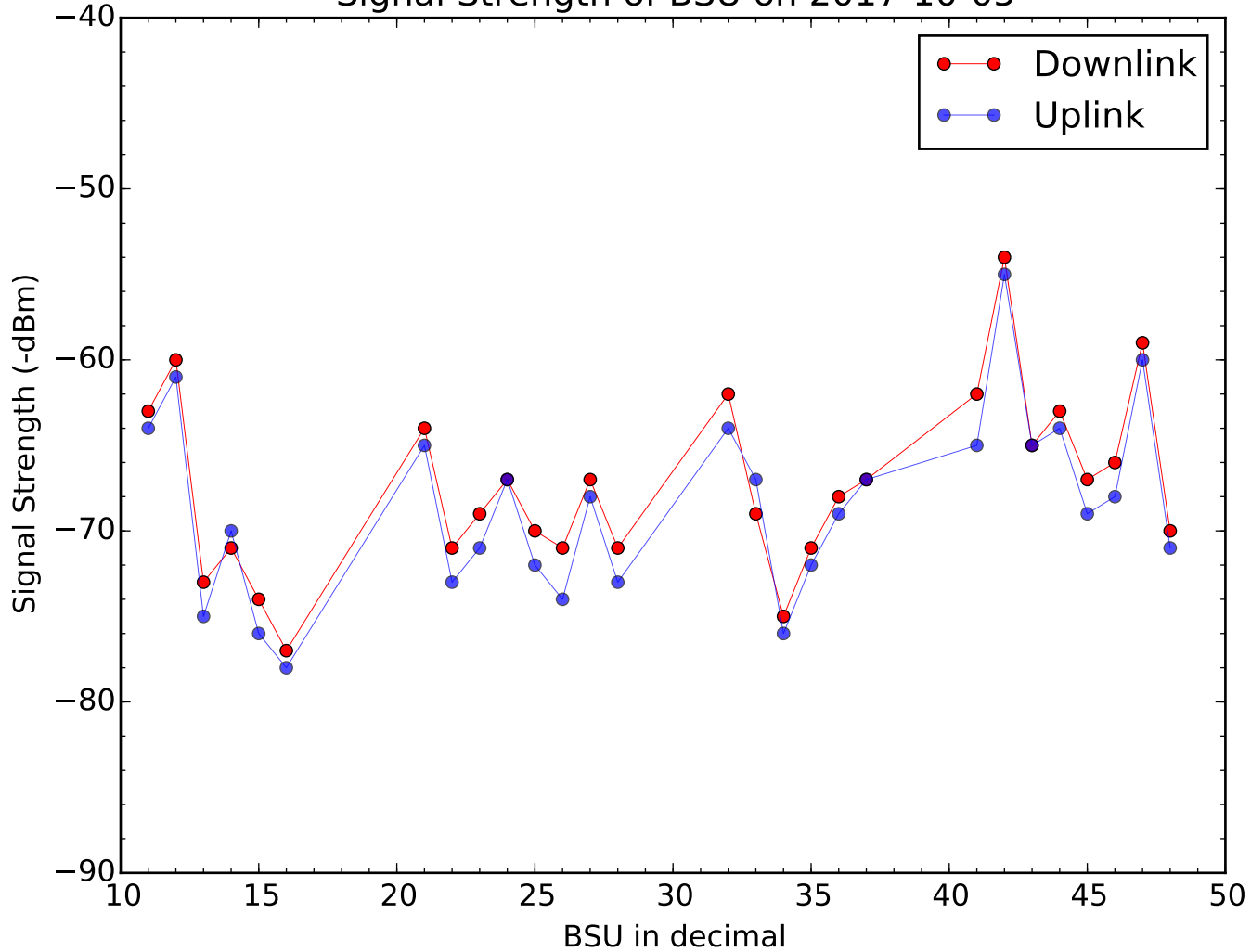
Signal Strength of BSU on 2017-10-05
