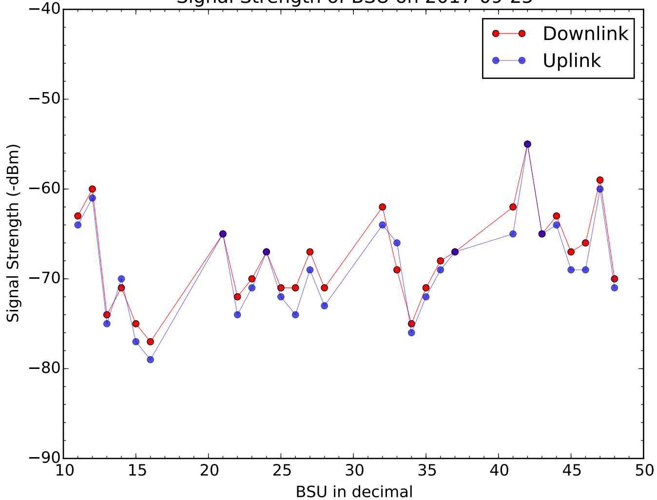
Signal Strength of BSU on 2017-09-25
