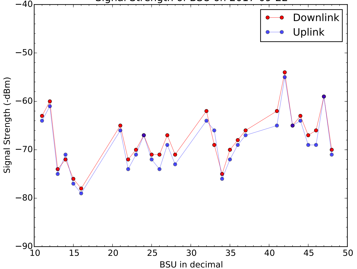
Signal Strength of BSU on 2017-09-22
