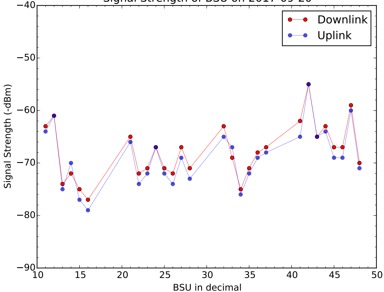
Signal Strength of BSU on 2017-09-20
