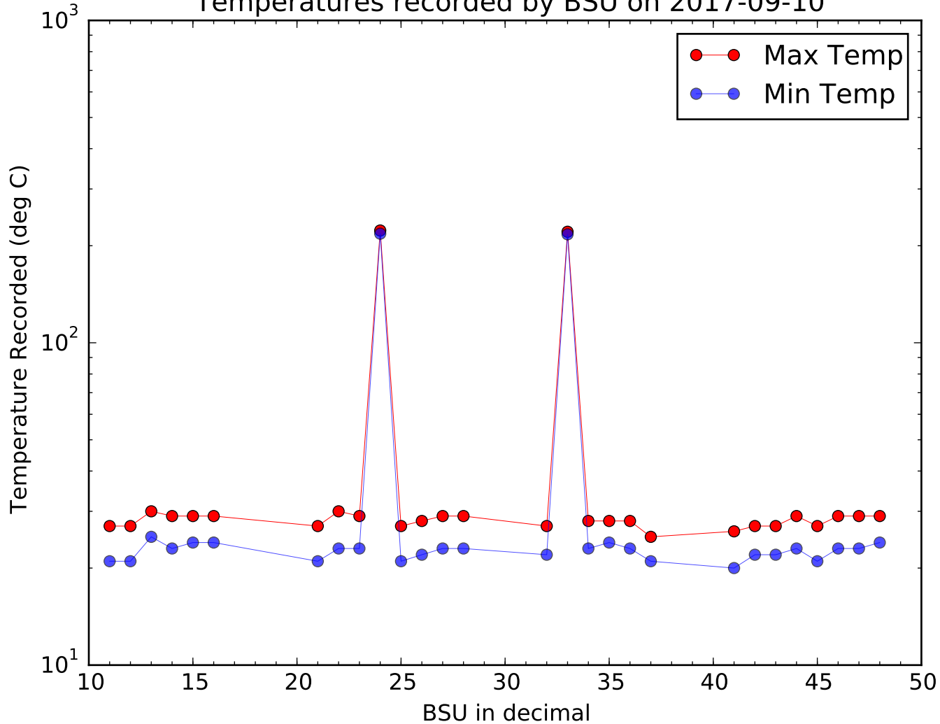
Temperatures recorded by BSU on 2017-09-10
