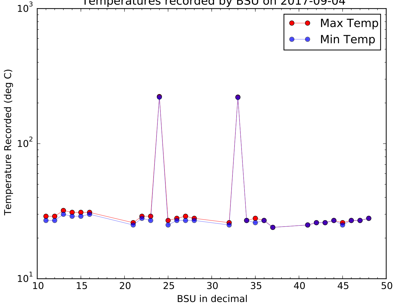
Temperatures recorded by BSU on 2017-09-04
