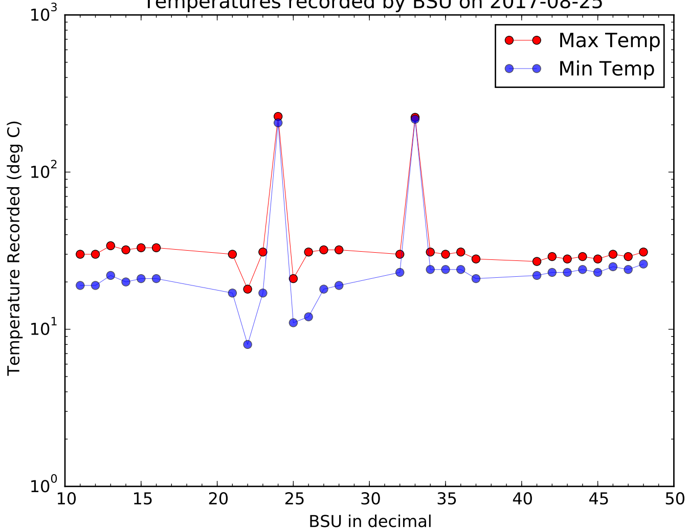
Temperatures recorded by BSU on 2017-08-25
