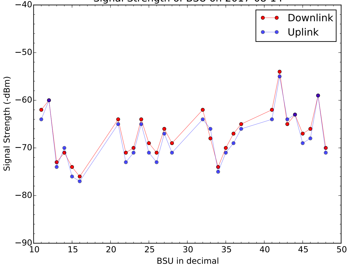
Signal Strength of BSU on 2017-08-14
