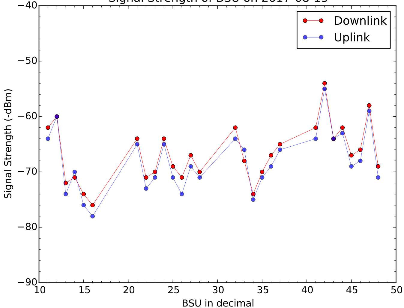
Signal Strength of BSU on 2017-08-13
